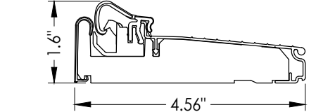
19 INSWING ARTICULATING THRESHOLD ZAC4565FN
