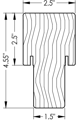
2A INTEGRAL MULLION FrameSaver (Endura)
