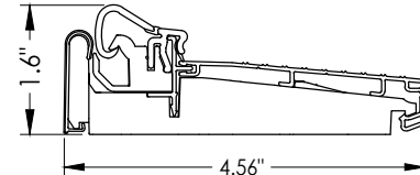
22 INSWING ARTICULATING THRESHOLD ZAC4565RDS
