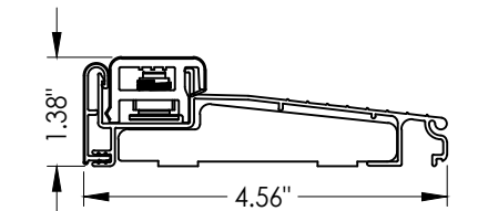
13 INSWING ADJUSTABLE THRESHOLD ZAIL4565
