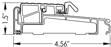
23 OUTSWING THRESHOLD ZOB4565
