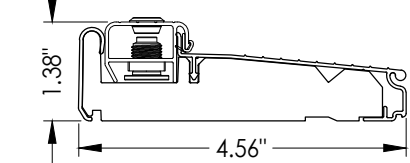
16 INSWING ADJUSTABLE THRESHOLD ZAI4565FN
