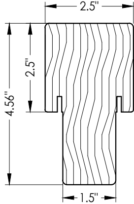
2 INTEGRAL MULLION
