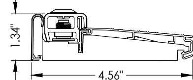
17 INSWING ADJUSTABLE THRESHOLD ZAI4565RDS
