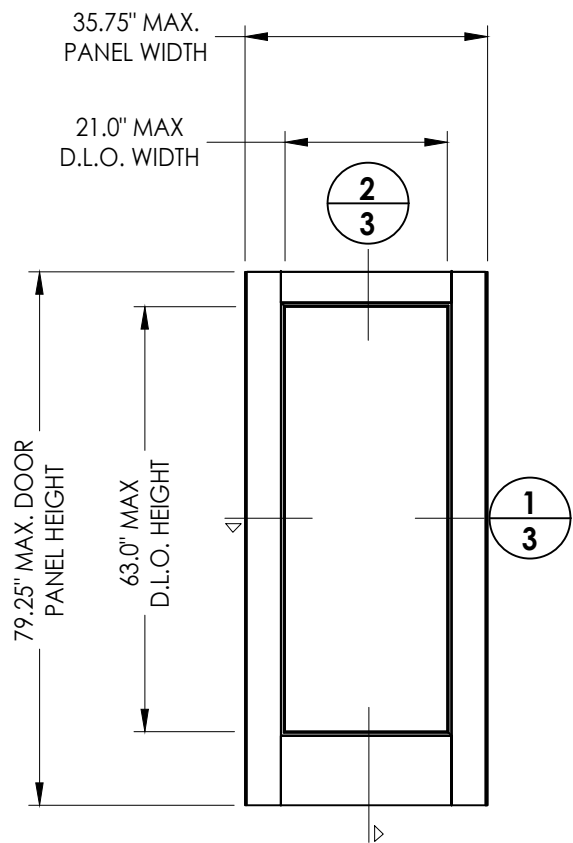
50 SIDELITE PANEL Masonite Fiberglass
