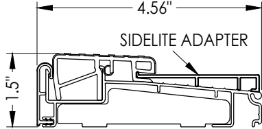
61 OUTSWING THRESHOLD w/ SIDELITE ADAPTER Endura (Z-Series)
